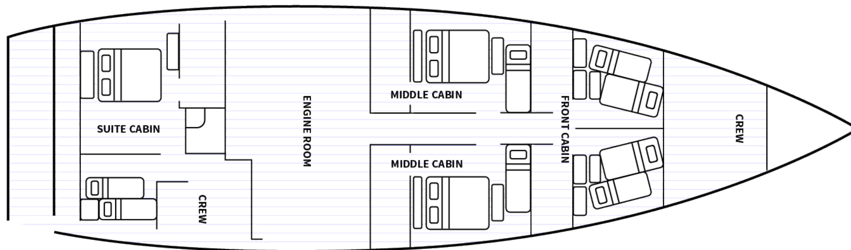
UPPER DECK
