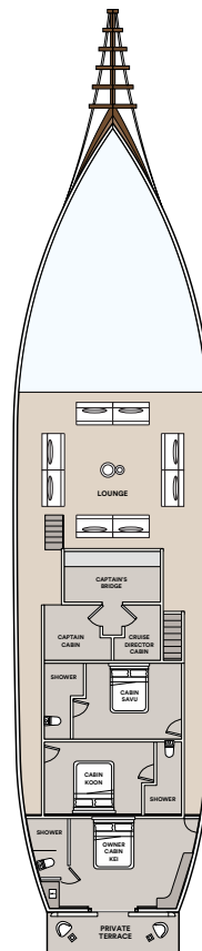
UPPER DECK
