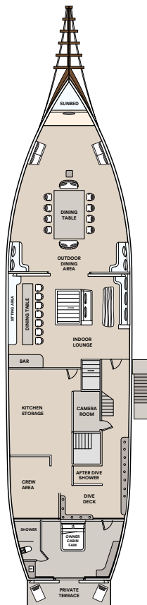
MAIN DECK
